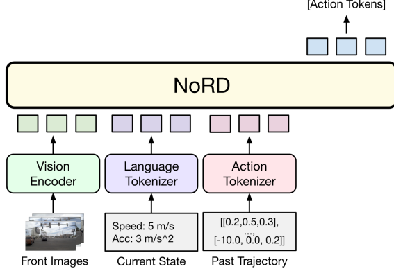
Figure 5. Model architecture of NORD. NORD directly predicts action tokens without requiring reasoning traces, enabling a significantly more efficient training and inference pipeline.
